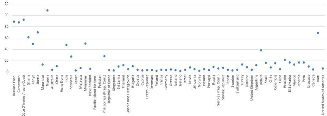
SDG 3.2.1: Under 5 mortality rate - Number of children death (per 1000 live births)
